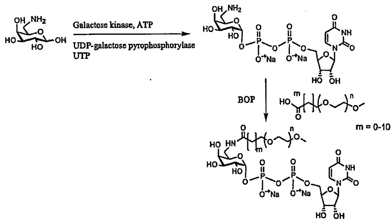
Scheme 10
